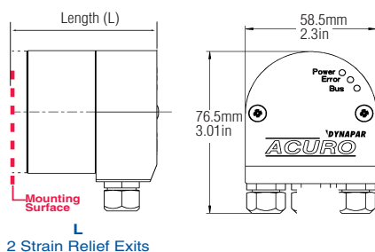
Length (L) Mounting Surface to Rear For connector types L, and F
