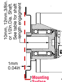
3 Hubshaft w/Tether
