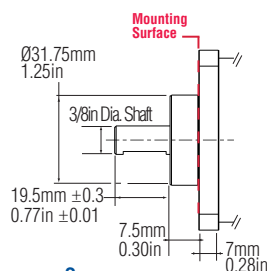
2 Square Flange
