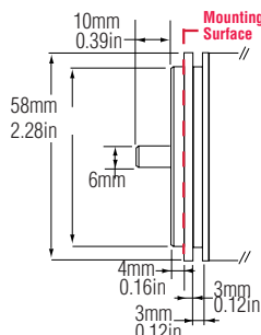
Code 3: Mounting
