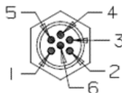
Male 6-Pin M8 (Code A)
