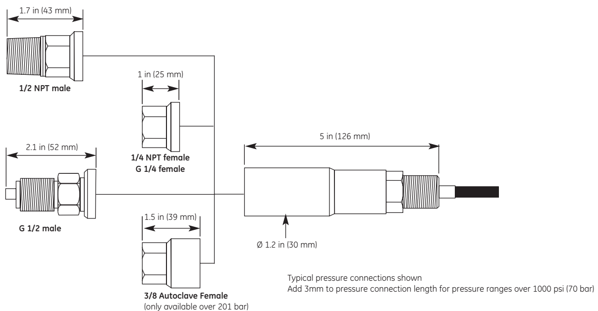
PTX 7800 Series dimensions
