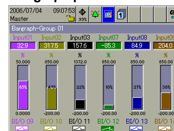
Bar graph presentation of analog channels
